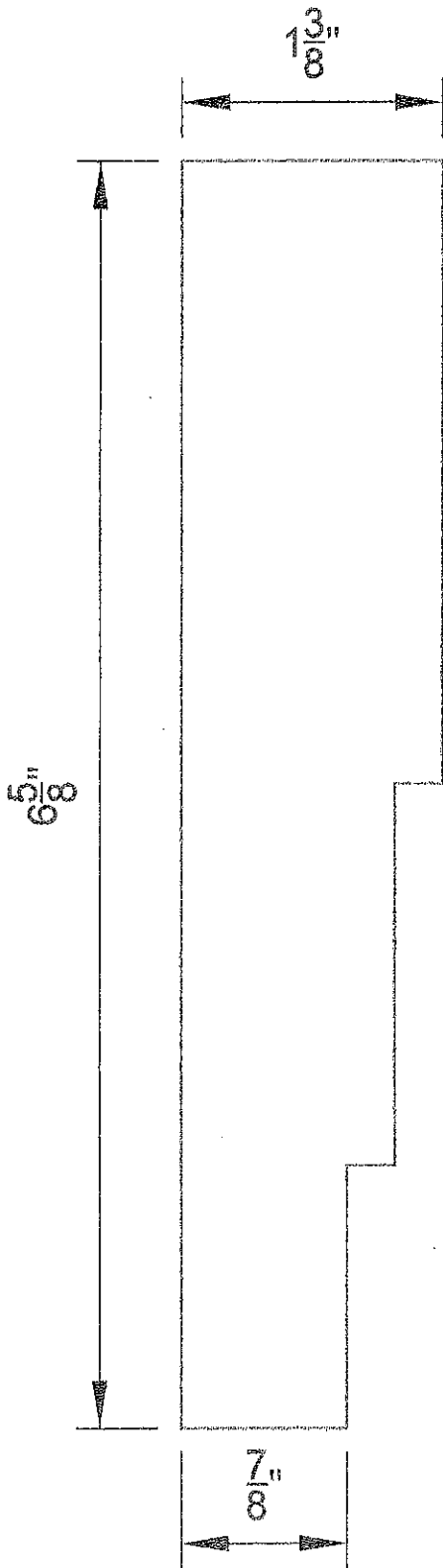
FASCIA BOARD
