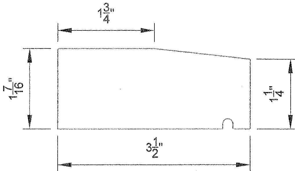
DRIP CAP
