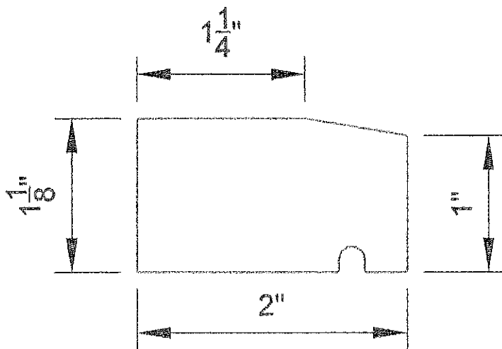
DRIP CAP - SILL EXTENSION
