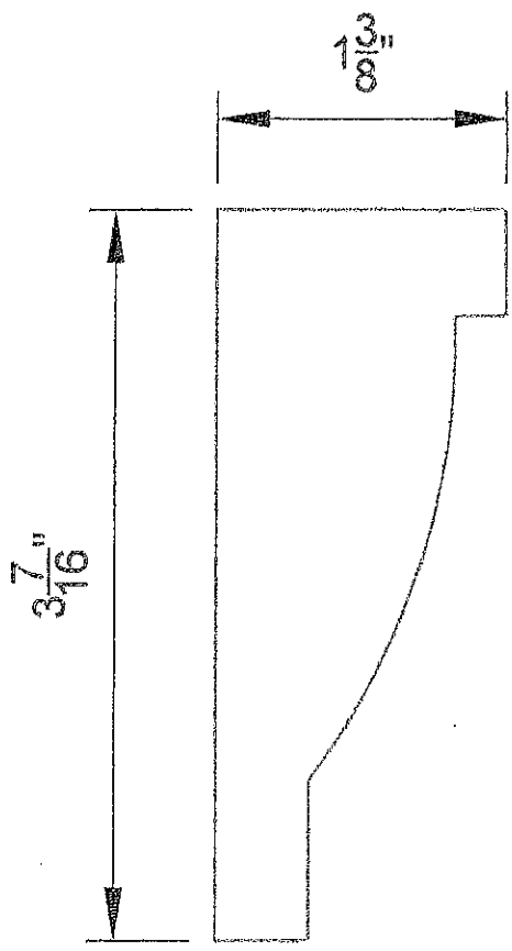
RAKE MOULDING
