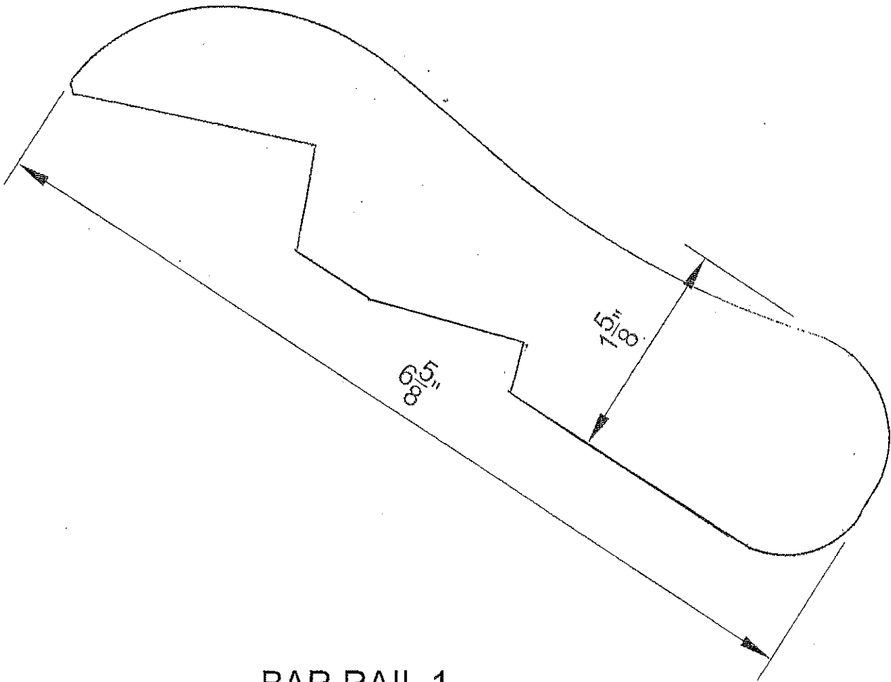
BAR RAIL 1
