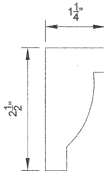
RAKE MOULDING
