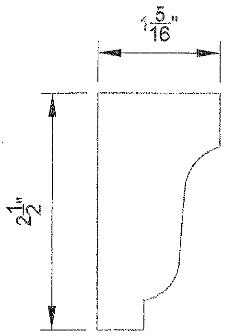
RAKE MOULDING
