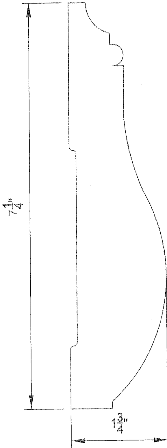
MANTEL SURFACE TRIM
